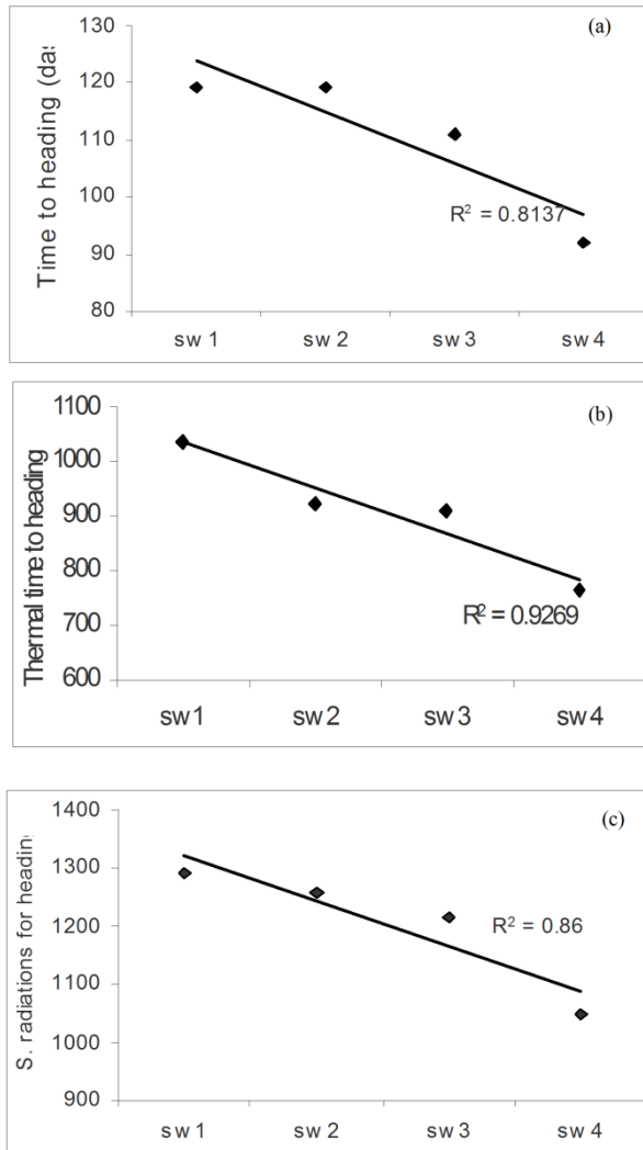
Figure 3: Relationship between (a) the times from sowing to heading (b) thermal time required from sowing to heading and (c) solar radiations required for heading and the sowing windows
