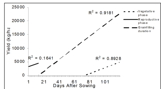
Figure 5: Wheat yield and duration of different growth phases
