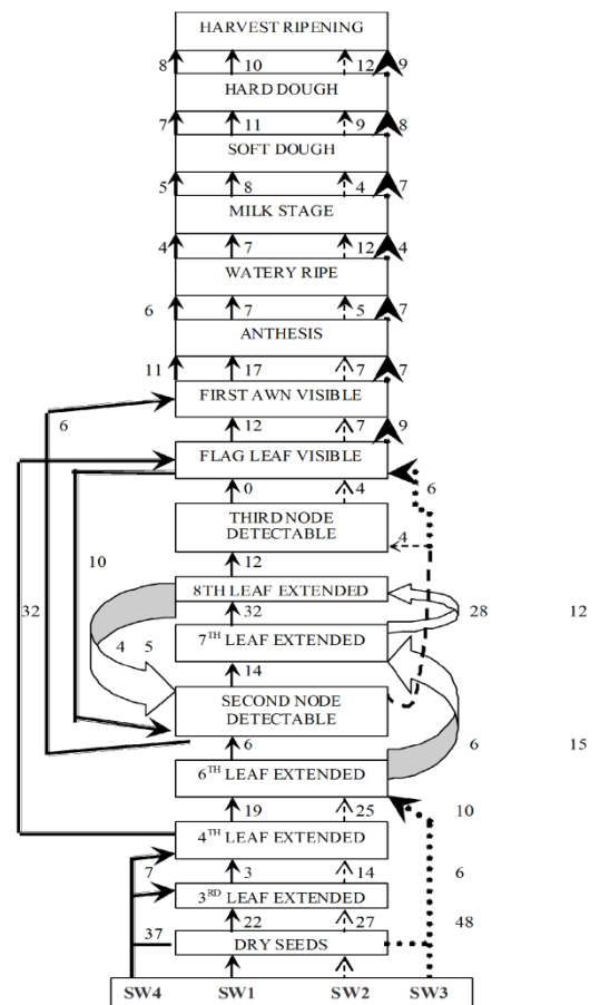
Figure 2: Pattern of Wheat Growth under different Sowing Windows. Numbers show the duration in days between growth stages
