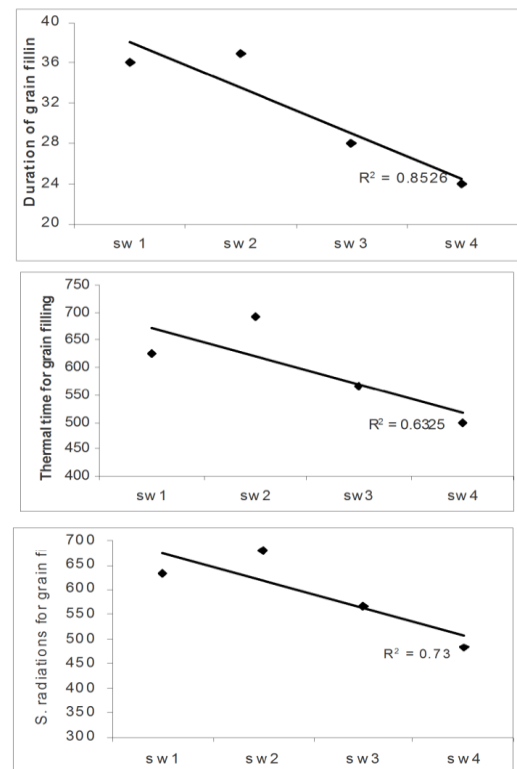
Figure 6: Relationship between (a) the duration of Grain Filling (b) Thermal Time required for grain filling and (c) Solar Radiations required for grain filling and the sowing windows.
