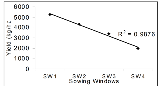
Figure 4: Wheat Yield under different sowing windows
