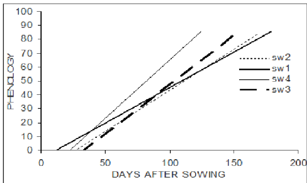
Figure 1: Different Sowing Windows and Duration of Wheat Phenological Stages
