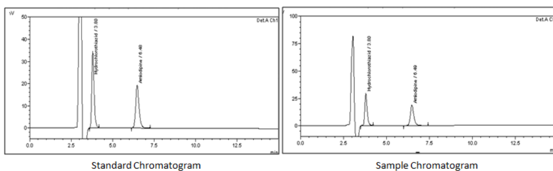
Fig. 1: Standard and sample chromatogram
