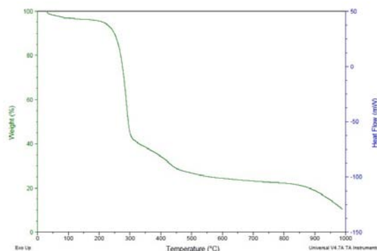
Fig. 3: TGA thermogram of optimized MTX FDT.
