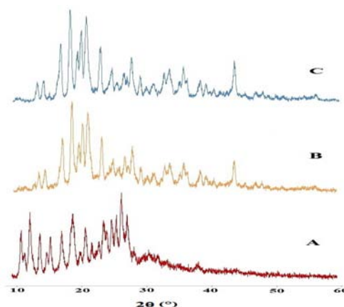
Fig. 4: X-ray diffractogram of pure drug (A), FDT formulation (B) and placebo tablet (C).
