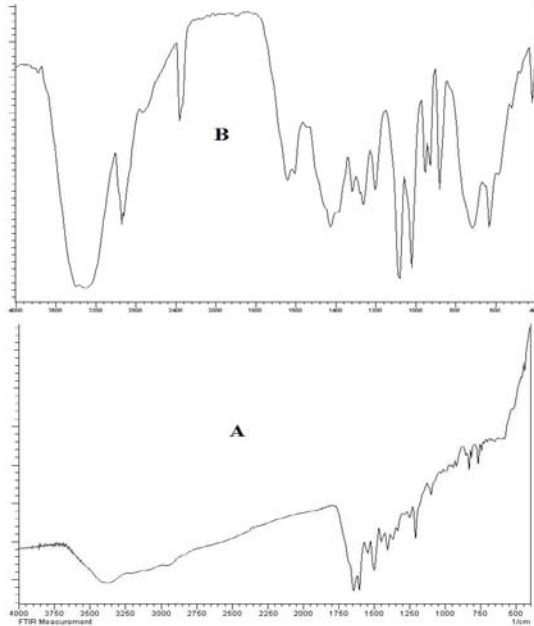
Fig. 1: FT-IR Spectra of pure Methotrexate (A) and Methotrexate-excipient physical mixture (B).
