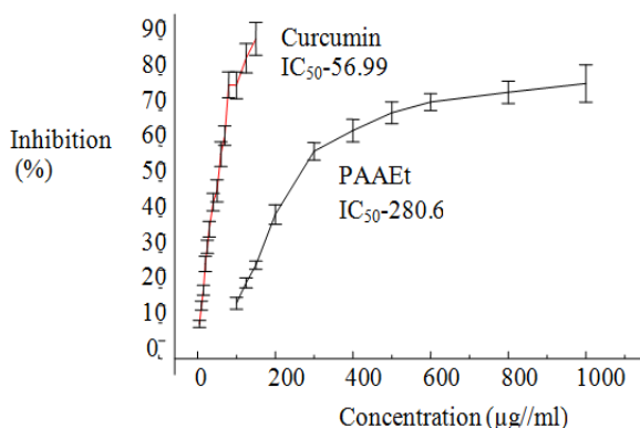
Fig. 1d: Hydroxyl radical scavenging activity of the PAAEt extract and the reference compound Curcumin
