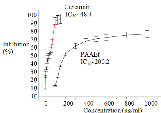
Fig. 1b: DPPH radical scavenging activity of the PAAEt extract and the reference compound curcumin
