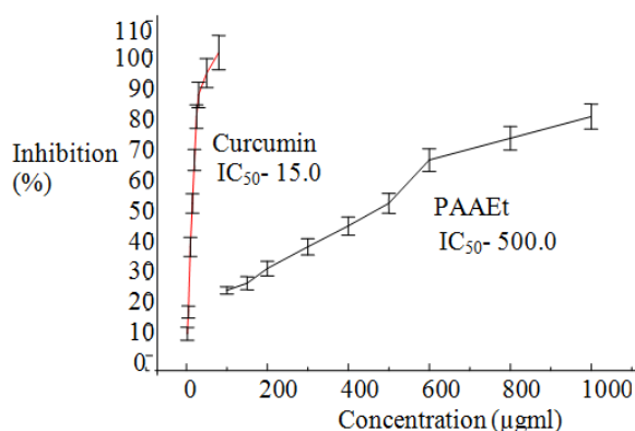
Fig. 1f: Reducing power activity of the PAAEt extract and the reference compound curcumin
