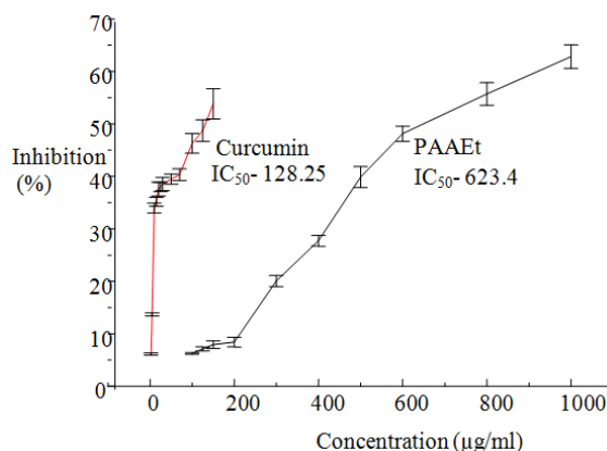
Fig. 1a: Lipid peroxidation inhibition activity of the PAAEt extract and the reference compound curcumin
