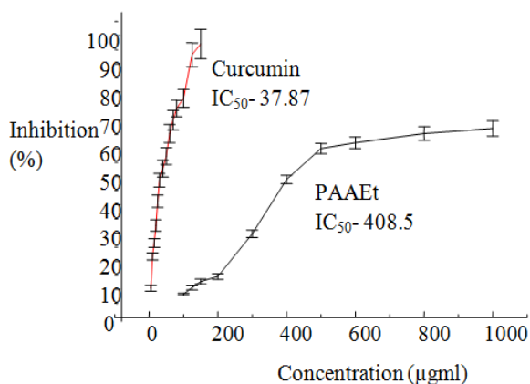
Fig. 1e: Nitric oxide radical scavenging activity of the PAAEt extract and the reference compound curcumin
