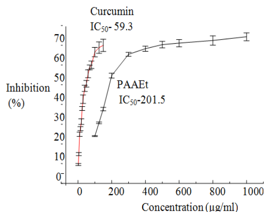
Fig. 1c: Superoxide radical scavenging activity of the PAAEt extract and the reference compound curcumin
